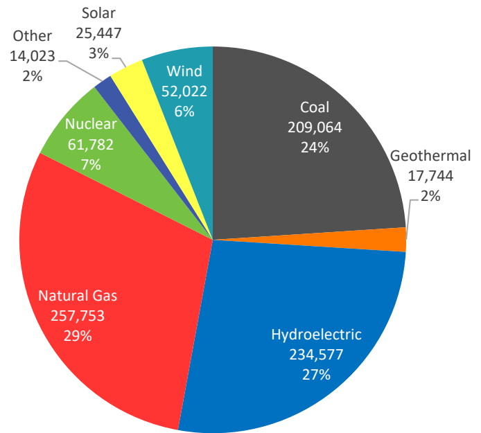
2016 Net Generation (GWh)
