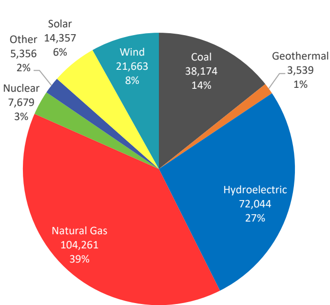
2016 Nameplate Capacity (MW)
