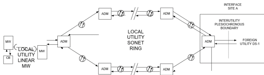
Figure 9 Terminated DS1
