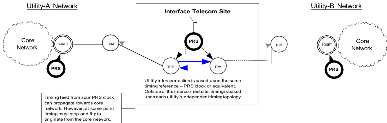
Figure 12 Inter-utility DS1 Interface Retiming
