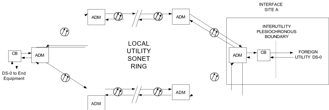
Figure 10 Terminated DS0
