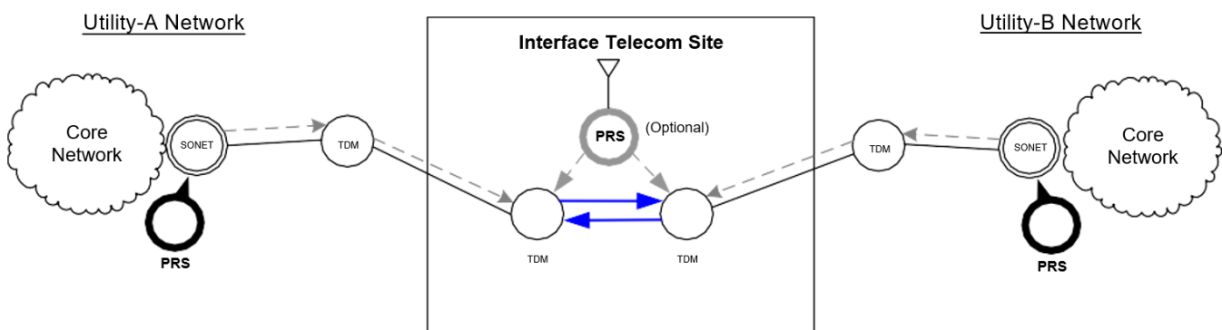
Figure 13 Inter-utility DS0 Interface PRS
