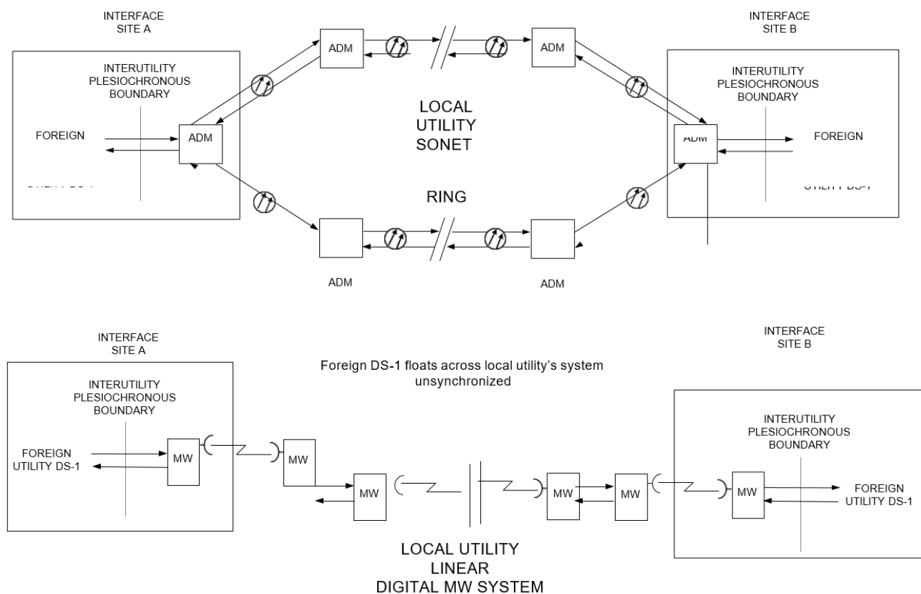
Figure 7 Floating DS1
