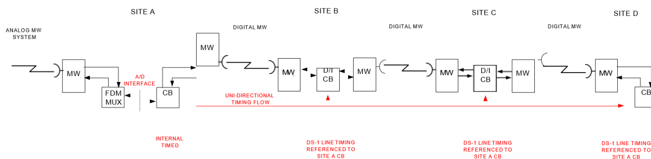
Figure 6 Isolated Linear MW System CB Timing
