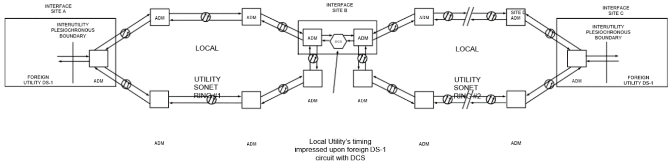
Figure 8 Intermediate Timed DS1
