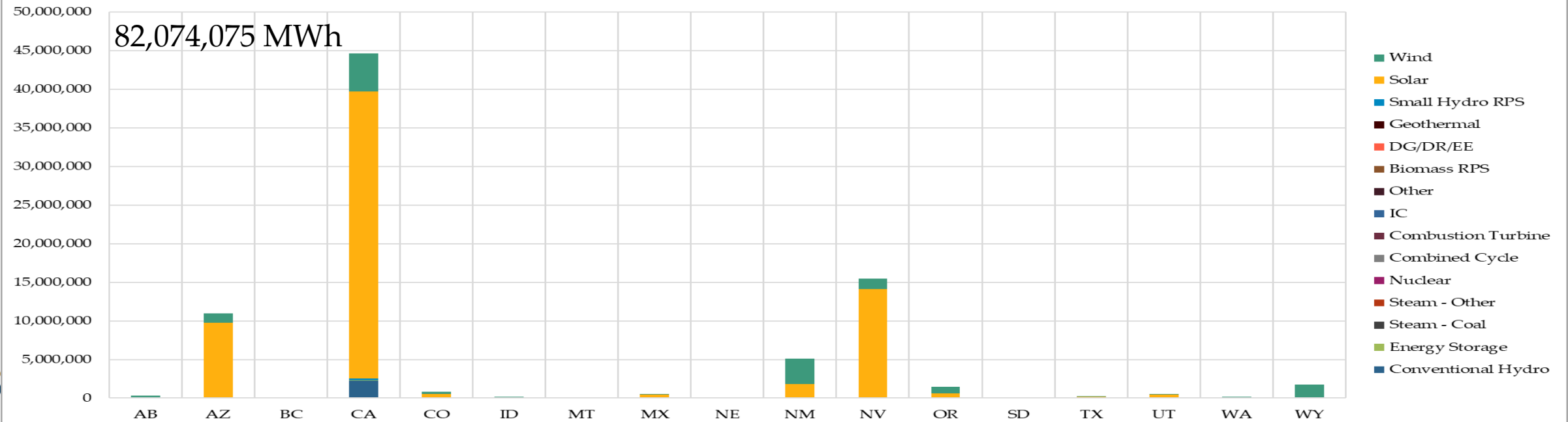
Annual Dumped Generation (MWh) by State and Type - 2034 ADS V2_12-9
