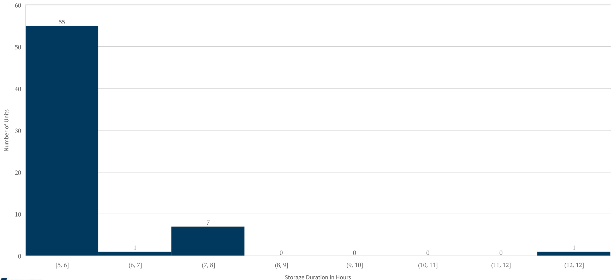
Storage Duration Histogram for added Storage in the 80% & 90% Clean Case
