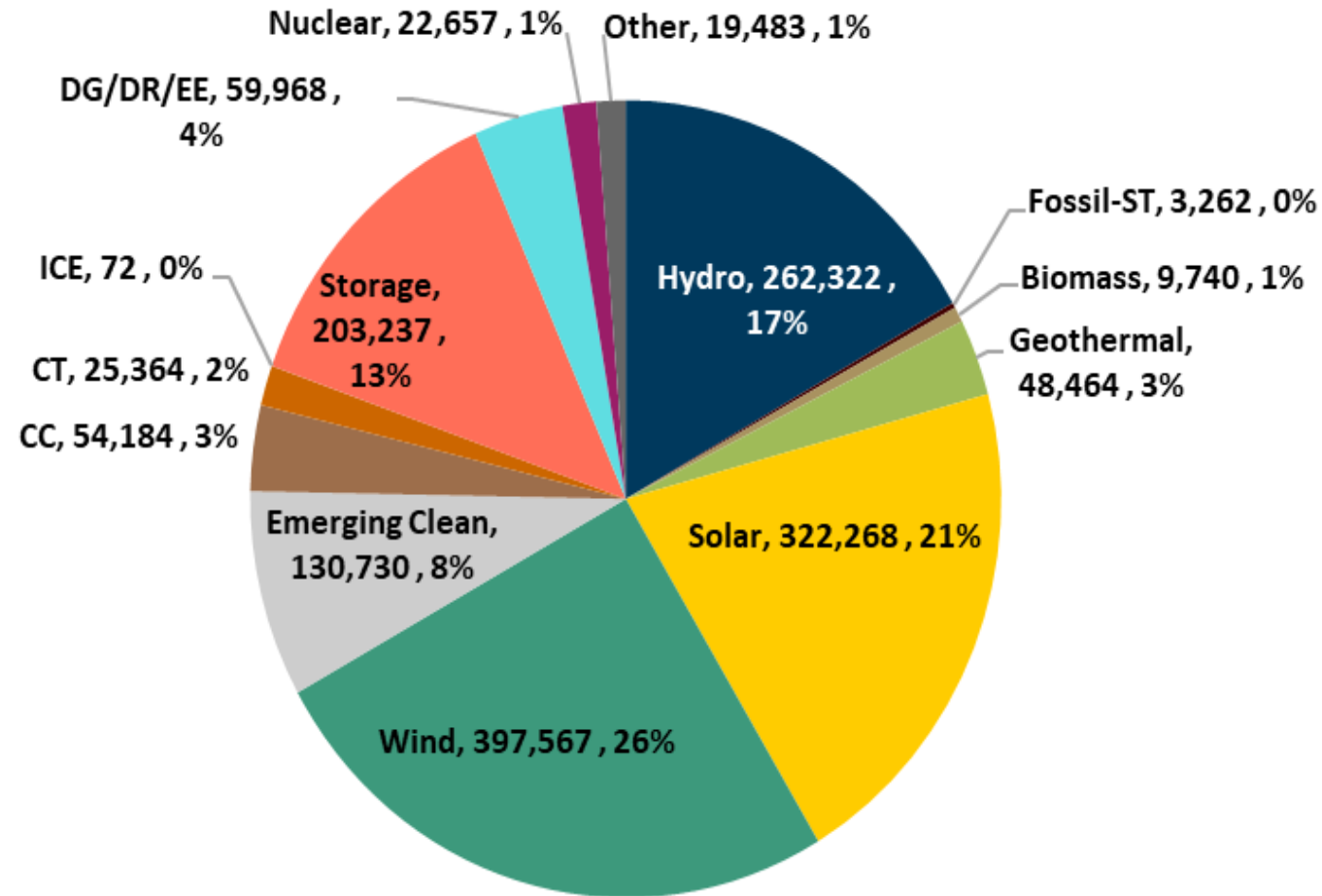
Energy Mix (GWh) by Gen Type – 2040 90% Clean
